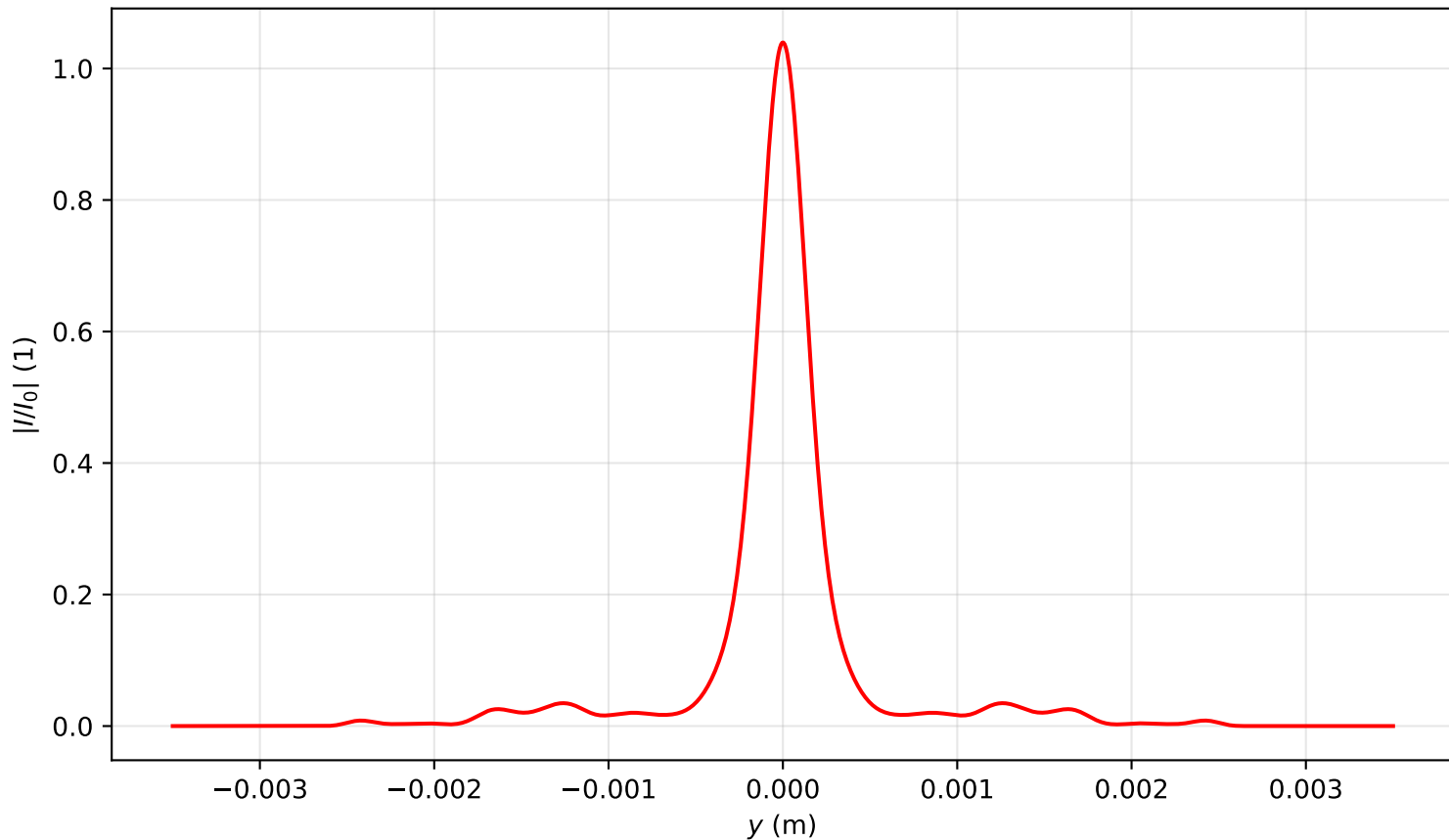
Intensity profile I(x=0, y, z=3.582)/I_0 , \text{Pin}=4.5\text{Pcr} , artificial time
